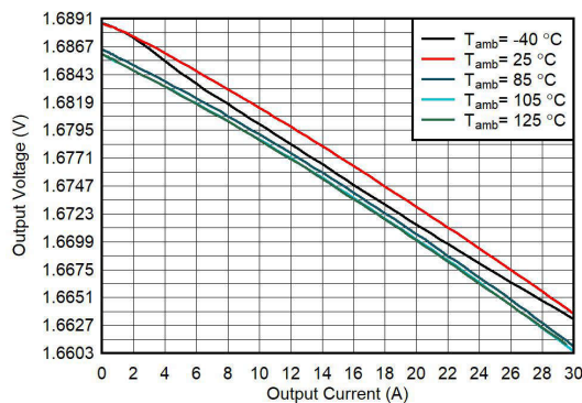
V_{IN} = 5.0V FPWM; TPS6287B25 V_{OUT} = 1.675V droop enabled
