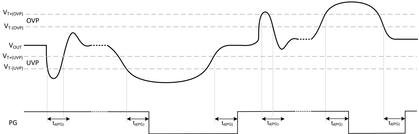
Figure 8-13. PG Timing
