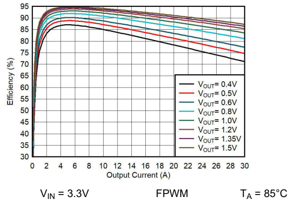
Figure 10-5. Efficiency vs Output Current
