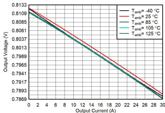
V_{IN} = 5.0V FPWM; TPS6287B25 V_{OUT} = 0.8V droop enabled
