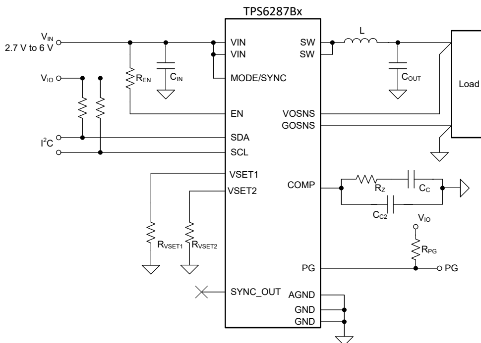
Figure 10-1. Typical Application Schematic
