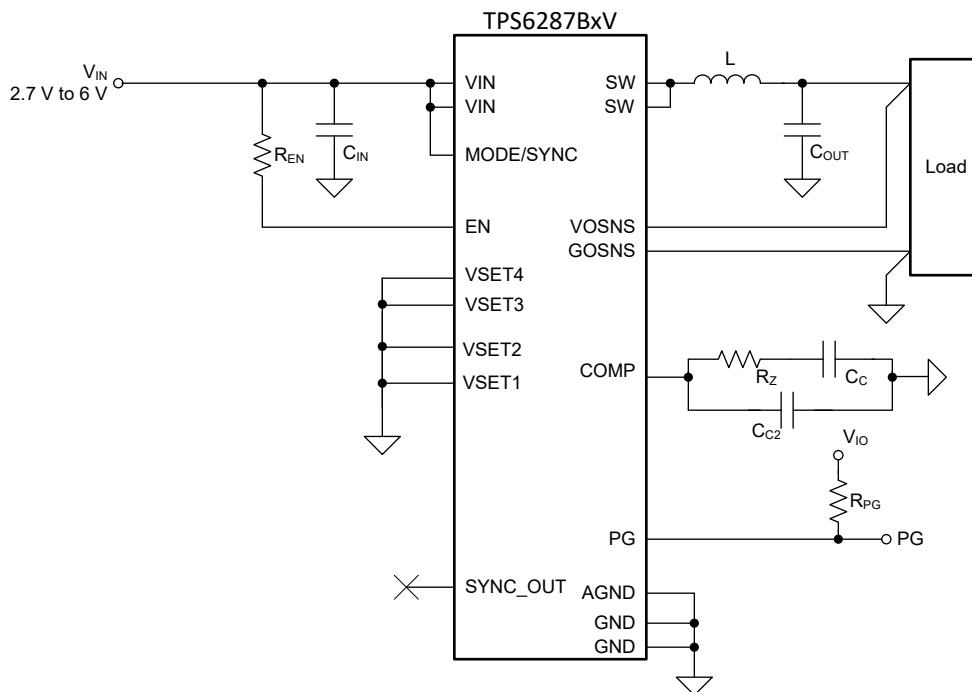
Figure 10-25. Typical Application Schematic for TPS6287BxV
