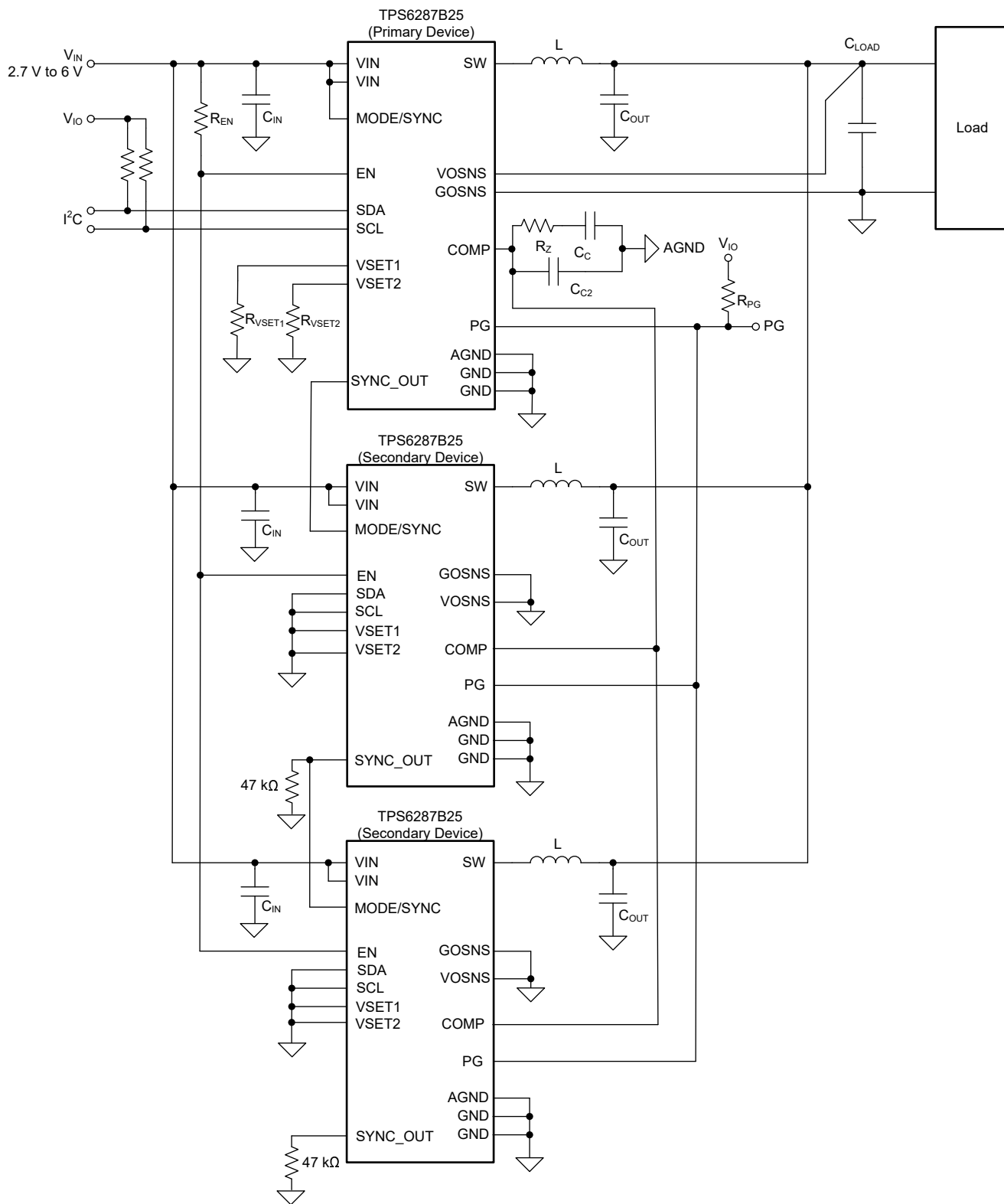
Figure 10-35. Stacking Three Devices
