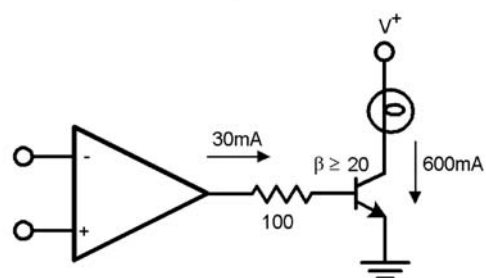
Lamp Driver
