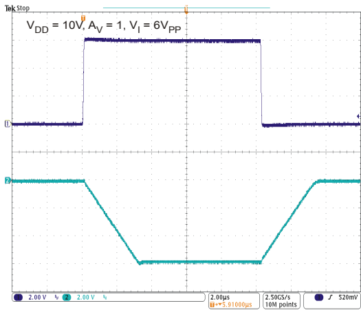
Figure 25 Inverting Large Signal Pulse Response V_{DD} = 10V
