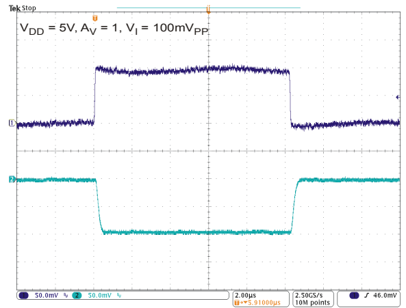
Figure 26 Inverting Small Signal Pulse Response
