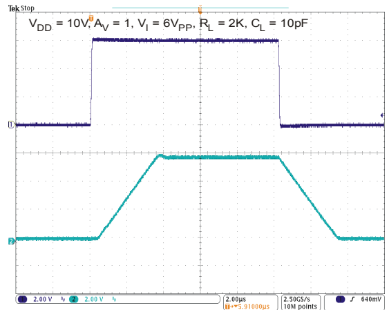
Figure 22 Voltage Follower Large Signal Pulse Response V_{DD} = 10V
