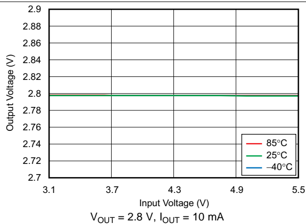
Figure 5. Line Regulation
