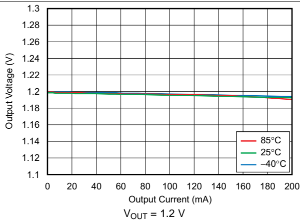
Figure 1. Load Regulation
