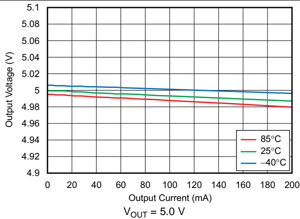
Figure 3. Load Regulation
