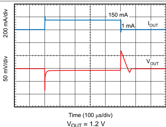
Figure 41. Load Transient Response
