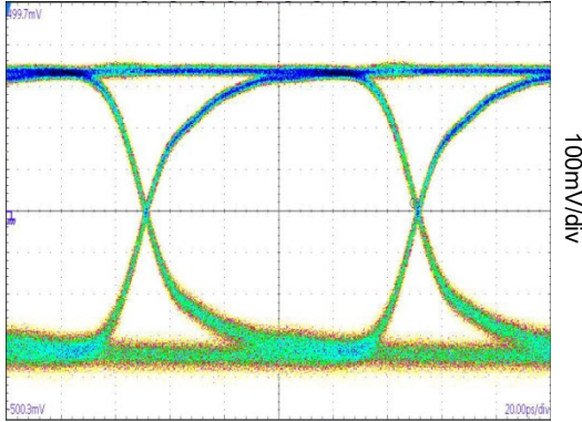
Time (20ps/div)
