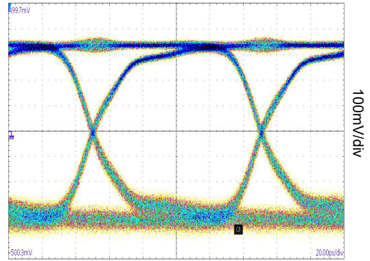
Time (20ps/div)
