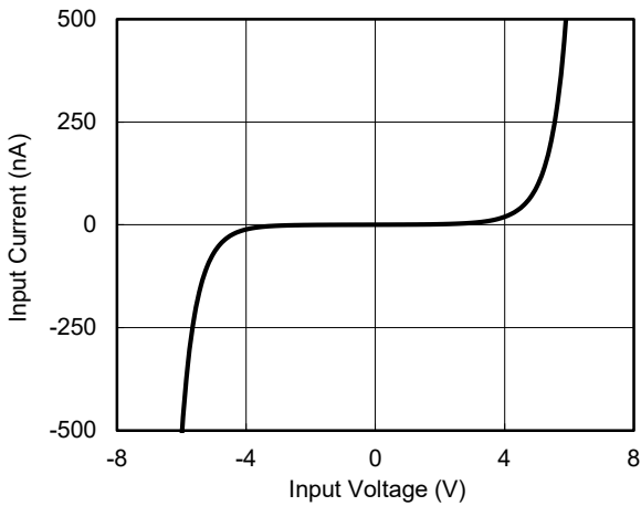
IV Curve
