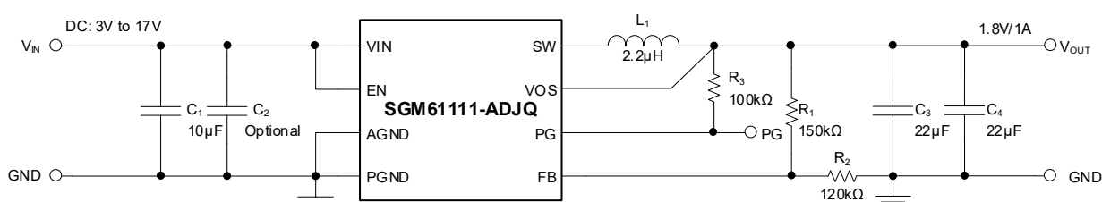
Figure 7. 1.8V Output Voltage Application of SGM61111-ADJQ
