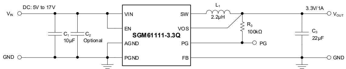
Figure 9. Application of SGM61111-3.3Q
