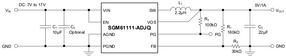
Figure 8. 5V Output Voltage Application of SGM61111-ADJQ
