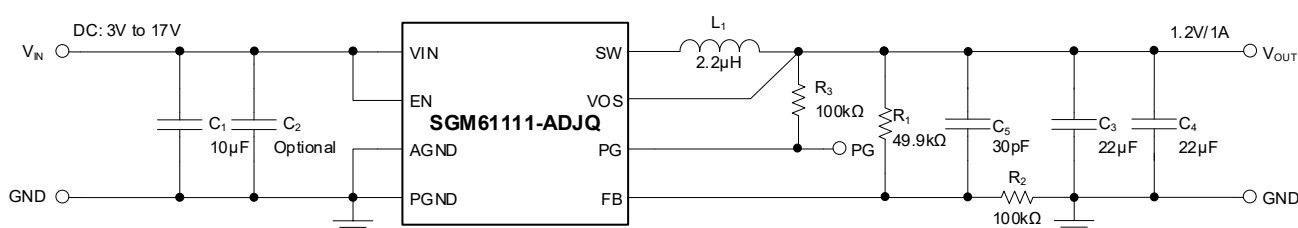
Figure 6. 1.2V Output Voltage Application of SGM61111-ADJQ
