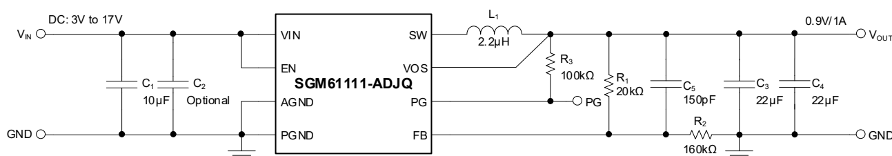
Figure 5. 0.9V Output Voltage Application of SGM61111-ADJQ
