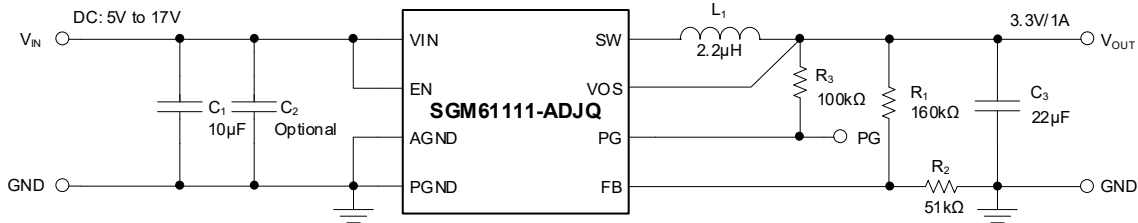
Figure 4. 3.3V Output Voltage Application of SGM6111-ADJQ
