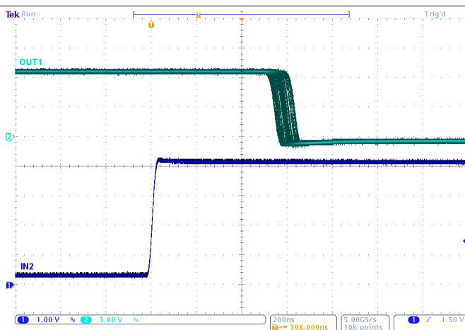
Figure 11. t_{PD}
