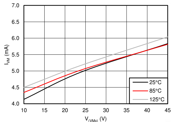
Figure 6-2. I VMx vs V VMx
