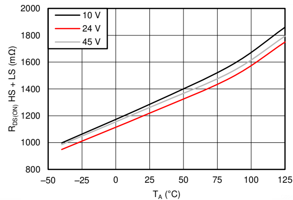
Figure 6-5. R DS(ON) vs Temperature
