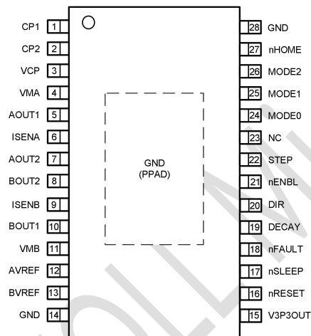
HTSSOP28(Top view) TMI8420
