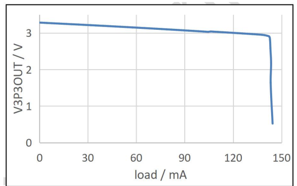
TMI8420/Q V3OUT3 Load Capacity
