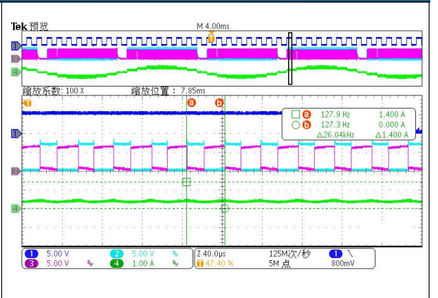
TMI8420/Q Fast decay waveform
