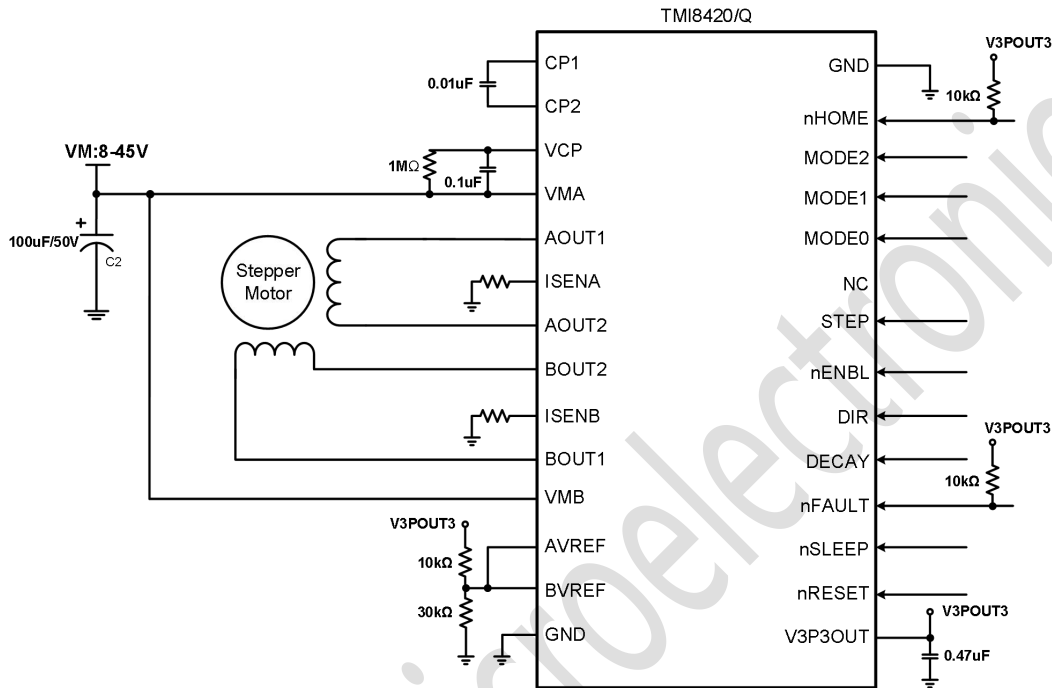
Figure 3. TMI8420/Q Typical Application
