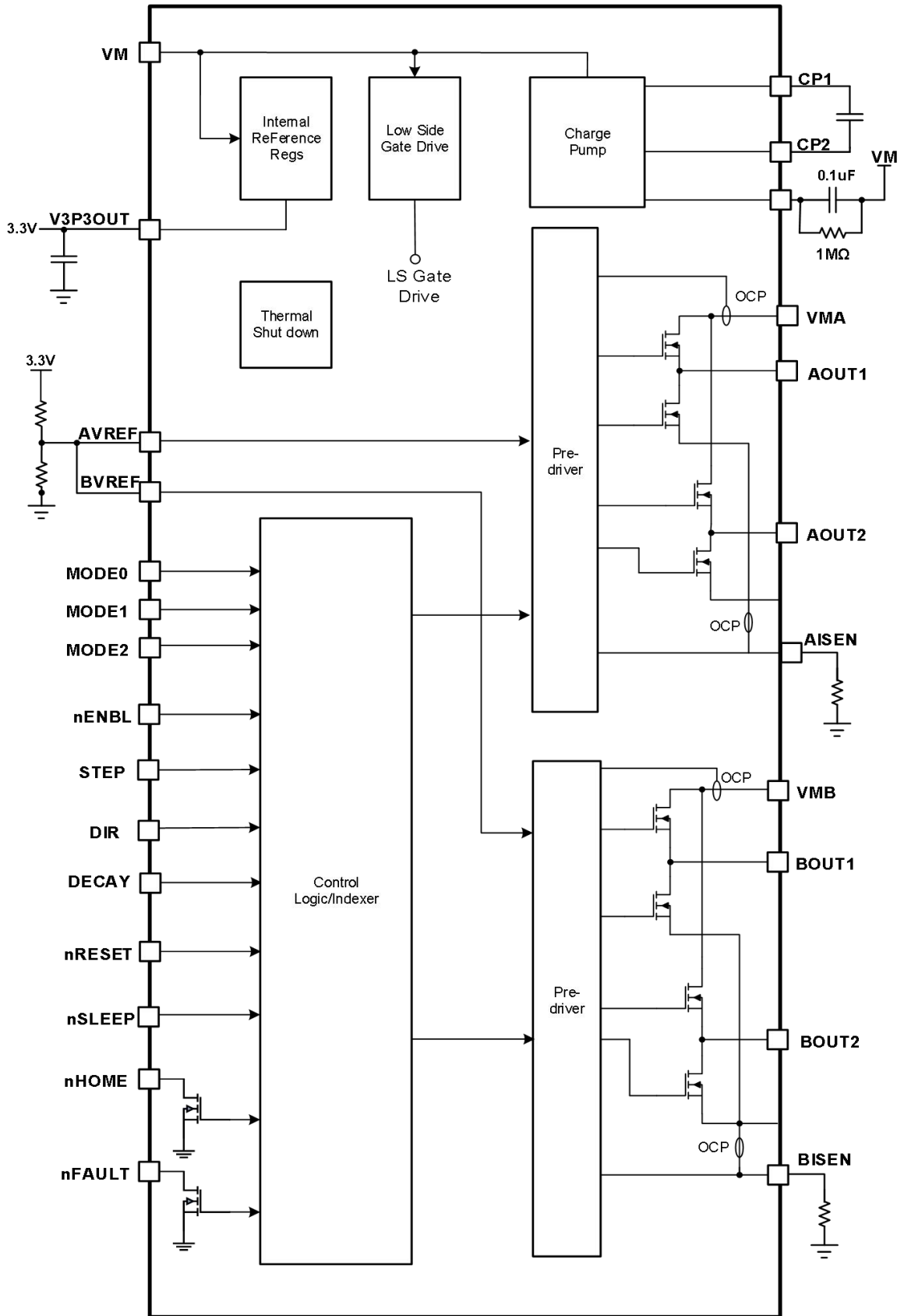
Figure 4. TMI8420/Q Block Diagram
