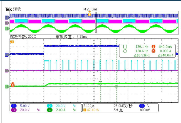
TMI8420/Q Slow decay waveform
