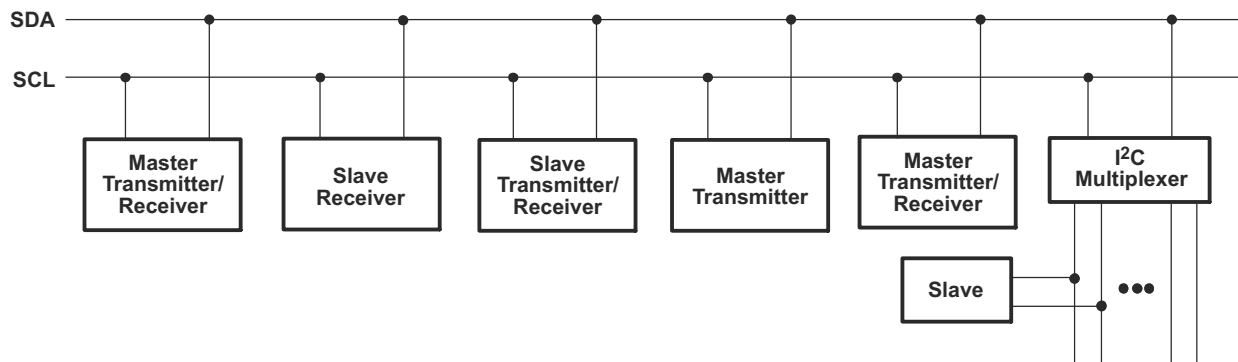
Figure 8-3. System Configuration
