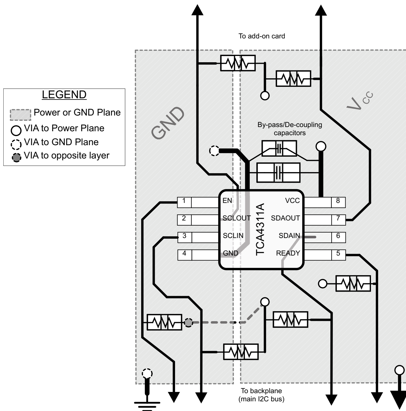
Figure 16. Package Layout
