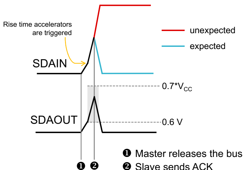
Figure 8. Missing ACK
