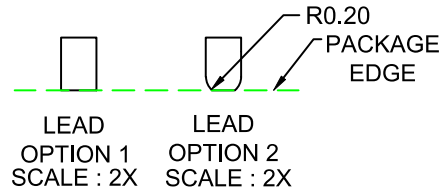
LEAD SHAPE AT PACKAGE EDGE
