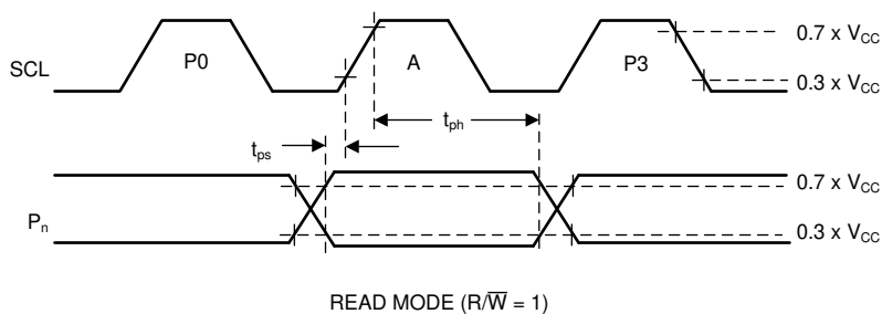
READ MODE ( R/\bar{W} = 1 )
