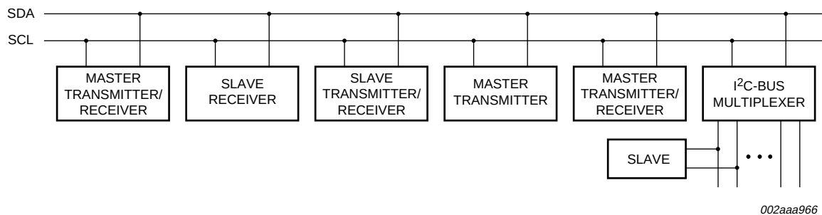
Fig 20. System configuration
