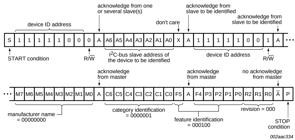
Fig 12. Device ID field reading
