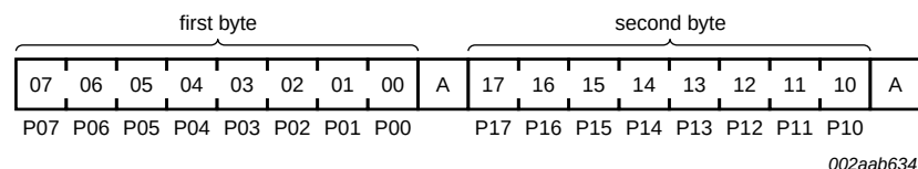
Fig 13. Correlation between bits and ports
