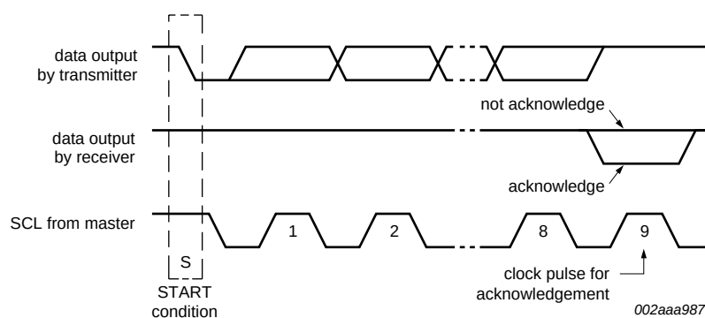
Fig 21. Acknowledgement on the I 2 C-bus
