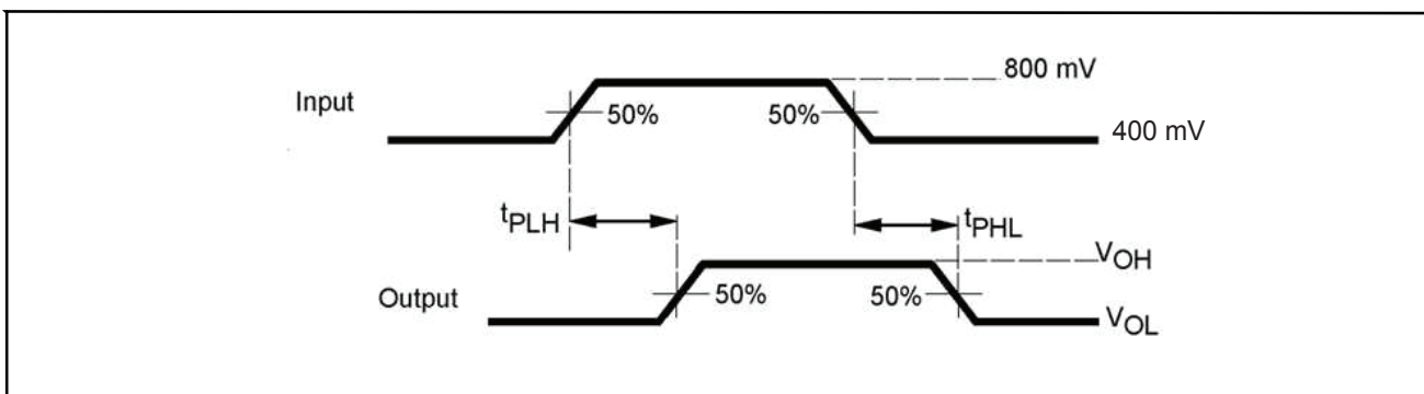
Figure 6. Propagation Delay
