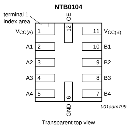
Fig 3. Pin configuration XQFN12 (SOT1174-1)
