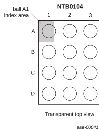
Fig 4. Pin configuration WLCSP12 package
