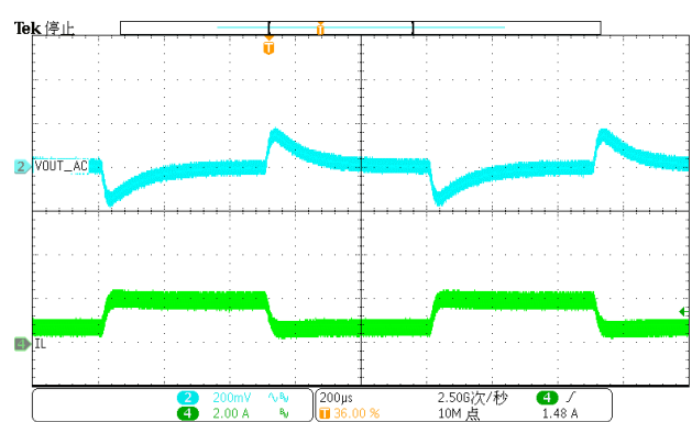
Figure 19. Load Transient (0.625A-1.875A, 1.6A/us)
