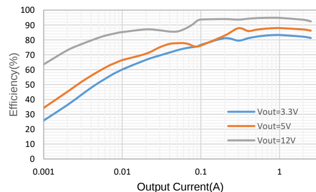
Efficiency, Vin=24V, Fsw=500KHz
