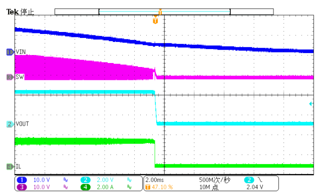
Figure 13. Power down(Iload=2.5A)
