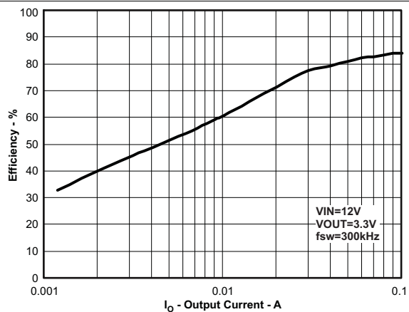
Figure 59. Light-Load Efficiency
