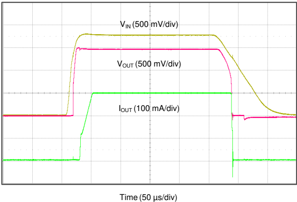
Figure 8-3. 1.8-V to 1.5-V Regulation at 300 mA
