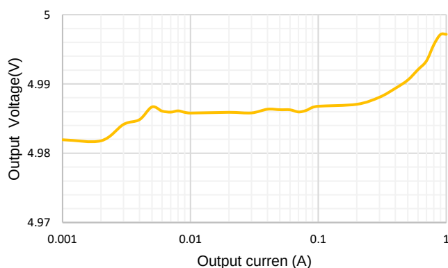
Figure 4. Load Regulation, Vin=24V, Vout=5V
