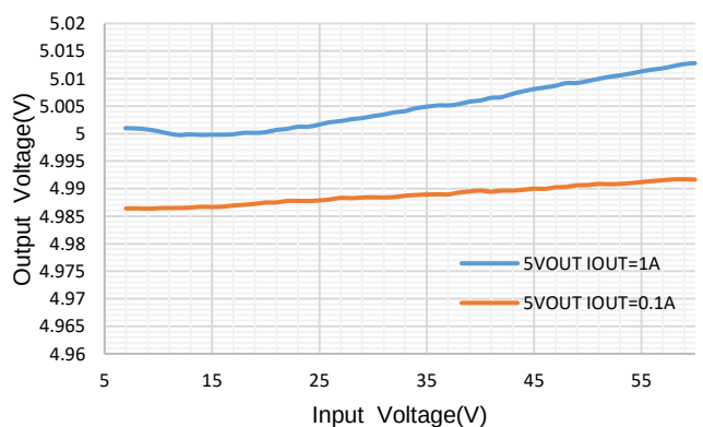
Figure 6. Line Regulation
