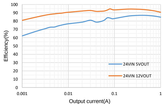
Efficiency, Vin=24V
