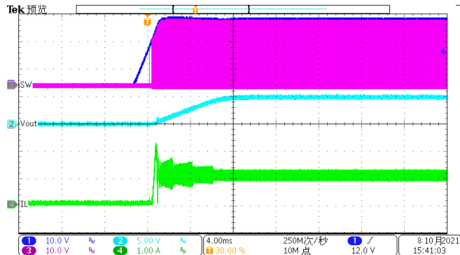
Figure 11. Power up(Iload=1A)
