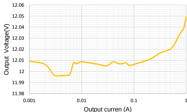
Figure 5. Load Regulation, Vin=24V, Vout=12V
