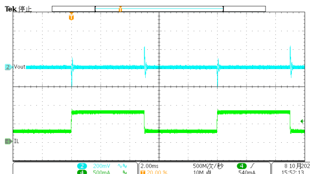
Figure 18. Load Transient (0.25A-0.75A, 1.6A/us)
