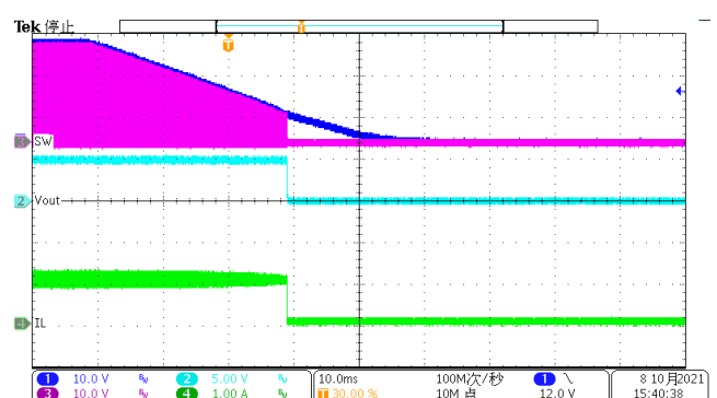
Figure 12. Power down(Iload=1A)
