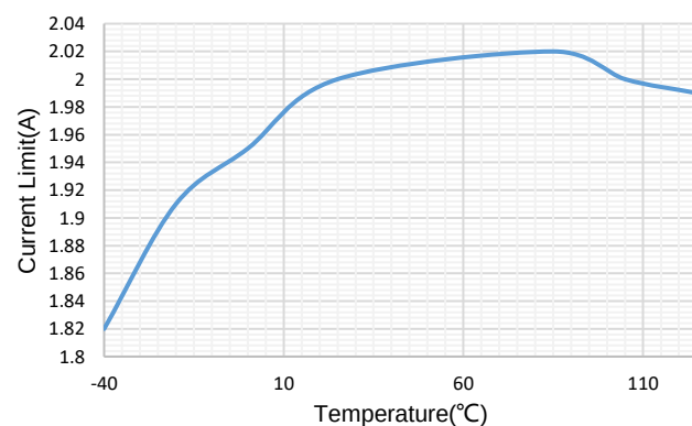
Figure 7. HS Current Limit VS Temperature
