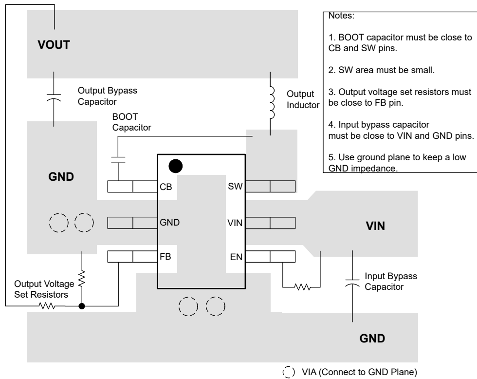
Figure 8-10. Layout
