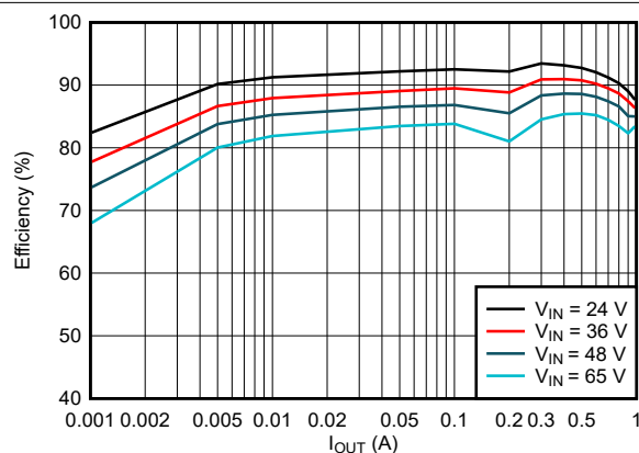
Figure 6-9. 5-V PFM Efficiency Versus Load Current
