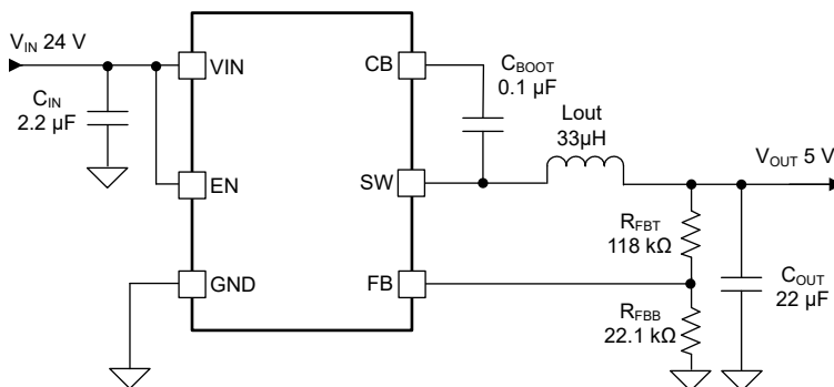
Figure 8-1. Application Circuit
