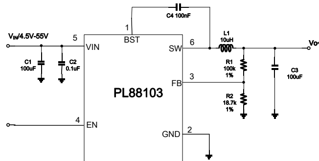
Fig 24 Schematic
