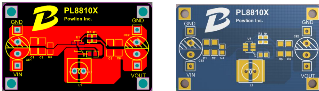
Fig 25 PCBLayout
