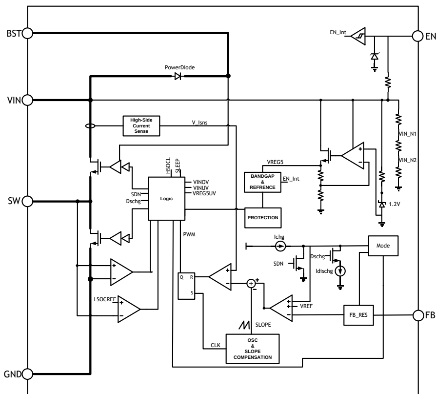
Fig.22 PL88103 Diagram
