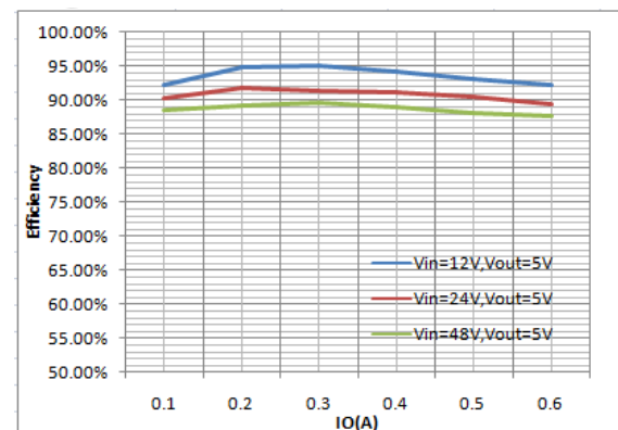
Fig. 2 Efficiency
