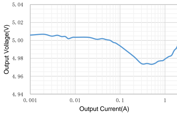
Figure 6. Load Regulation ( V_{IN}=24V , V_{OUT}=5V )
