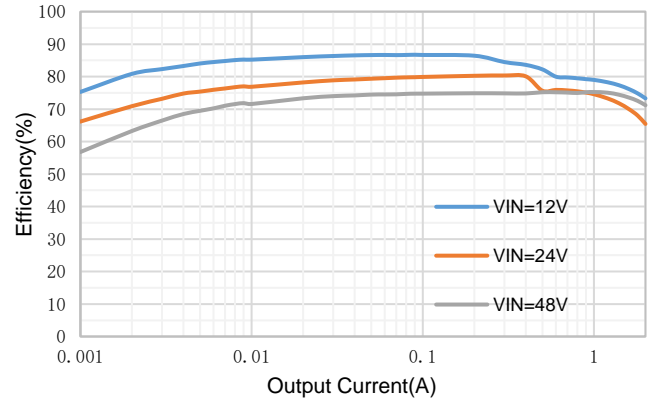
Figure 3. Efficiency, F_{SW}=2MHz , V_{OUT}=5V
