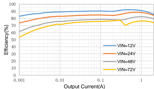
Efficiency, Fsw=400kHz, VOUT=5V
