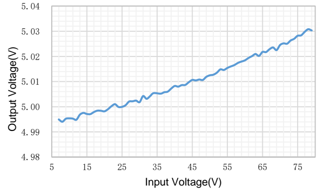
Figure 5. Line Regulation ( V_{OUT}=5V , I_{LOAD}=1A )
