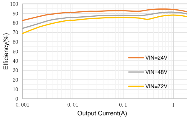
Figure 4. Efficiency, F_{SW}=400kHz , V_{OUT}=12V
