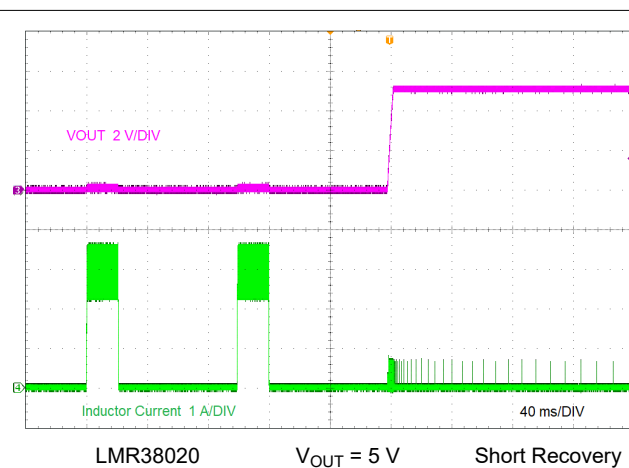
Figure 9-8. Short-Circuit Recovery
