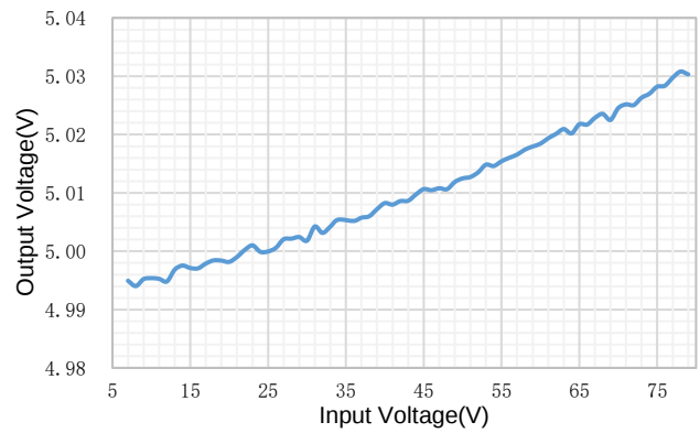
Figure 5. Line Regulation ( V_{OUT}=5V , I_{LOAD}=1A )
