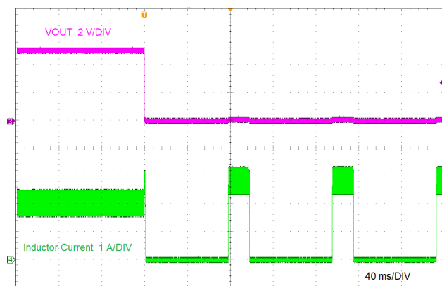
LMR38020-Q1 V_{OUT} = 5\text{ V} 2 A to Short
