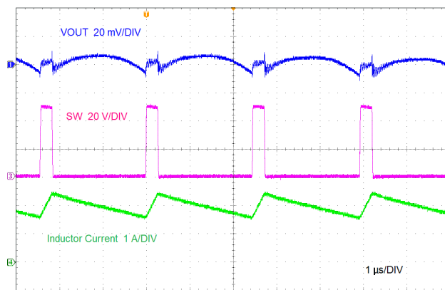
LMR38020-Q1 V_{OUT} = 5\text{ V} AC Coupled 400 kHz
