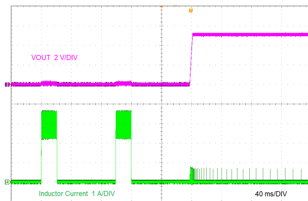
LMR38020-Q1 V_{OUT} = 5\text{ V} Short Recovery
