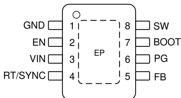
Figure 5-1. DDA Package, 8-Pin HSOIC (Top View)
