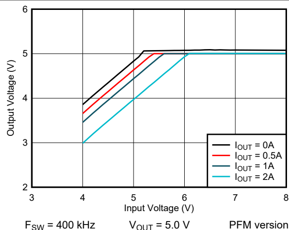
Figure 6-3. 5-V Dropout
