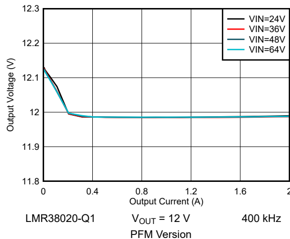
Figure 8-14. 12-V Load Regulation
