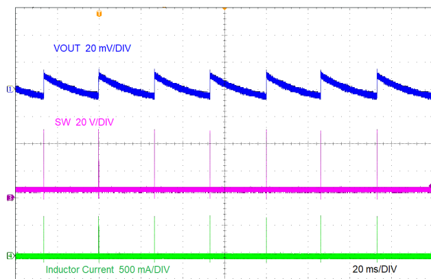
LMR38020-Q1 V_{OUT} = 5\text{ V} AC Coupled No Load
