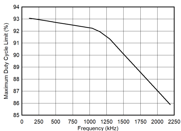
Figure 7-16. Maximum Duty Cycle Limit vs Frequency
