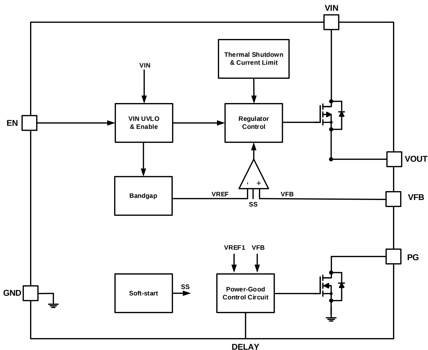
Figure 10. Functional Block Diagram of Adjust Output Version
