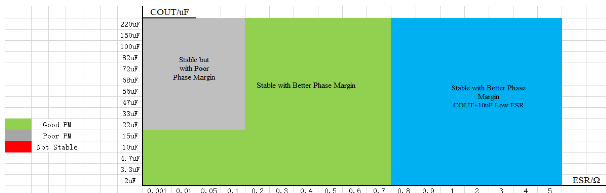
Figure 22. SCT71601 Stability VS Output Capacitor
