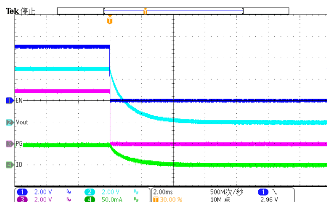
Figure 34. Disable (Iload=50mA)
