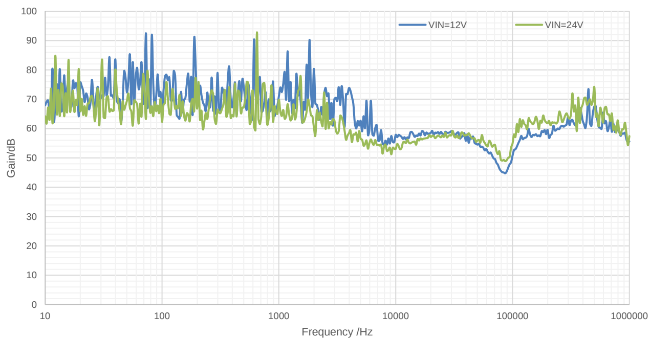
Figure 6. PSRR vs Frequency VOUT=3.3V,Cf=10pF,COUT=10uF,IOUT=10mA
