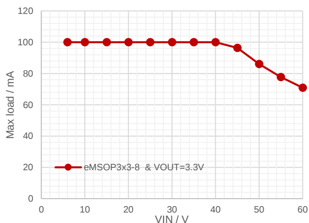
Figure 24. Maximum Output Current vs Input Voltage, VOUT=3.3V of eMSOP3X3-8, T_J \leq T_{SD\_R}
