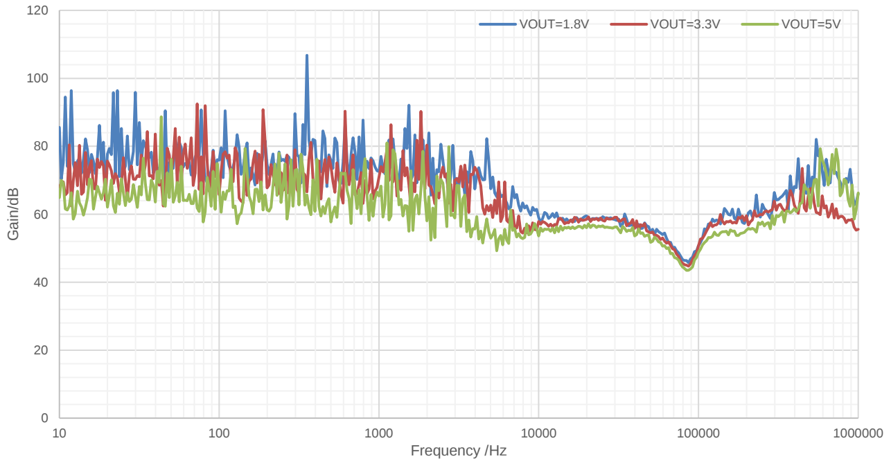
Figure 8. PSRR vs Frequency VIN=12V, Cf=10pF, COUT=10uF, IOUT=10mA
