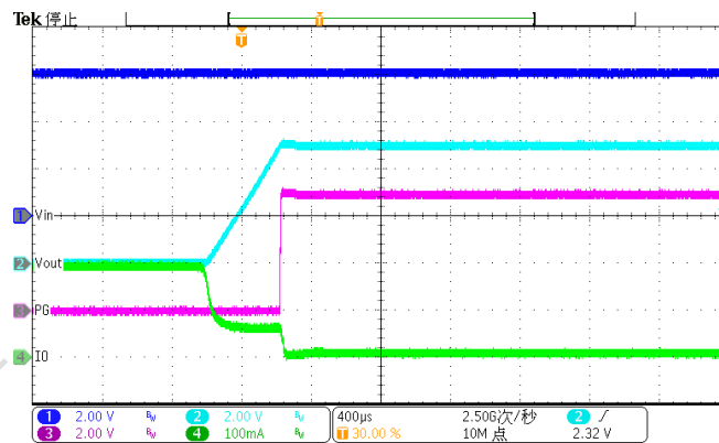
Figure 36. Exit Short Circuit Protection
