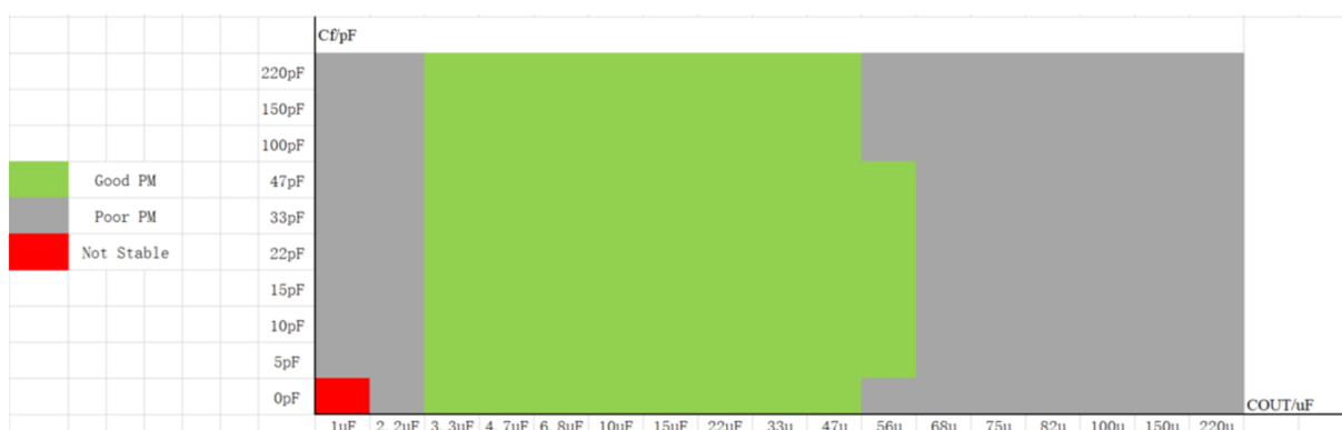
Figure 21. SCT71601 Feed Forward Capacitors recommend( R_2=10k\Omega , V_{OUT}=1.8V )
