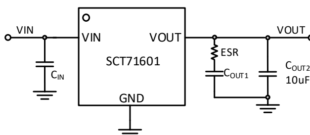
Figure 19. SCT71601 Typical Application Schematic with Large Output Capacitor
