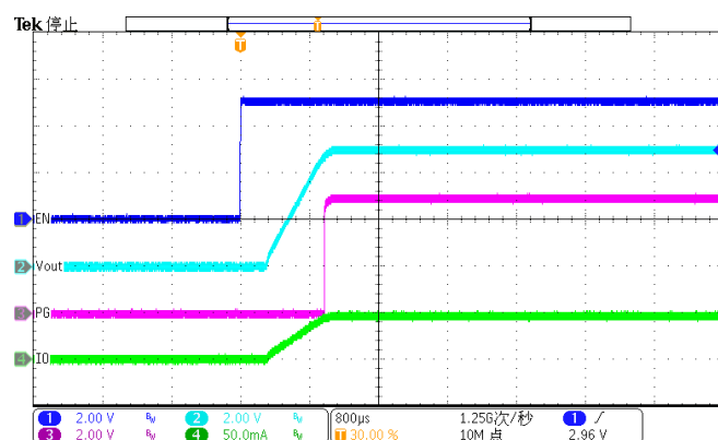
Figure 33. Enable (Iload=50mA)
