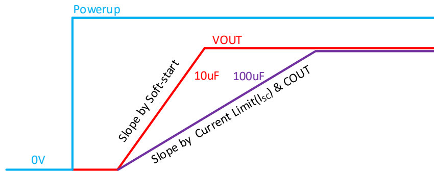
Figure 13. Soft-start Waveform vs Output Capacitor
