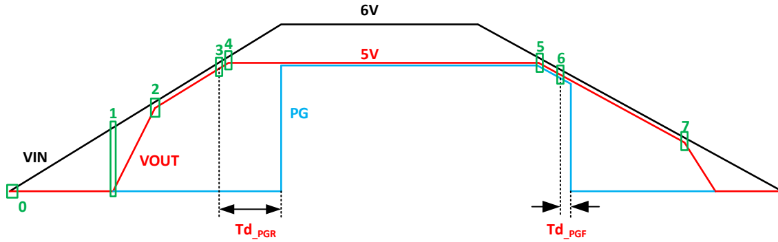
Figure 16. Startup and Shutdown Example —SCT71601 Series
