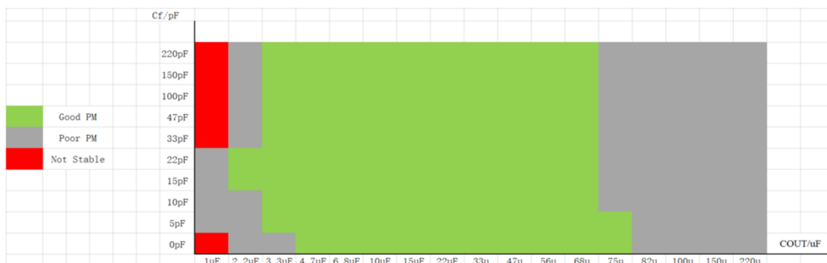
Figure 20. SCT71601 Feed Forward Capacitors recommend( R_2=100k\Omega , V_{OUT}=1.8V )
