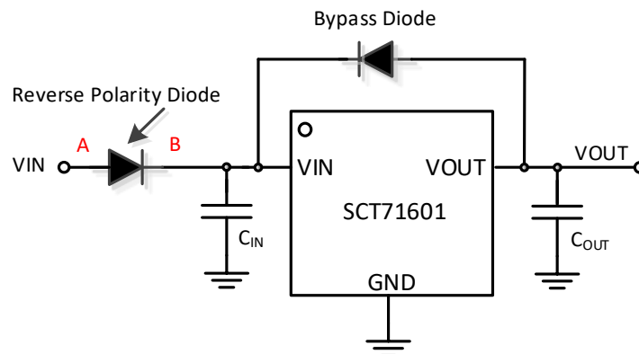
Figure 18. SCT71601 Typical Application Schematic with Reverse Polarity Diode
