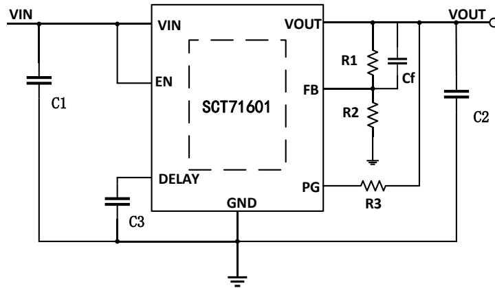
Figure 17. SCT71601 Typical Application Schematic
