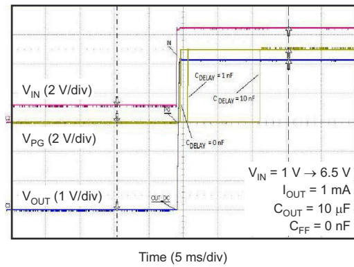
Figure 6-13. Power-Good Delay
