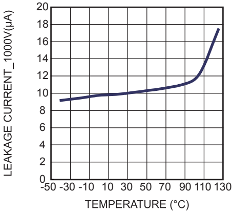
Leakage Current_1000V vs. Temperature Chart
