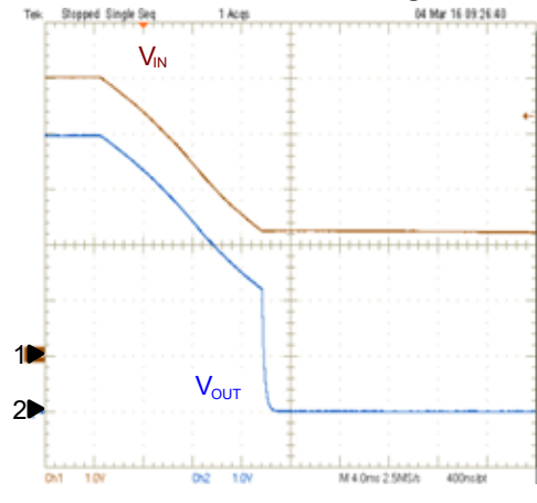
UVLO at Falling
