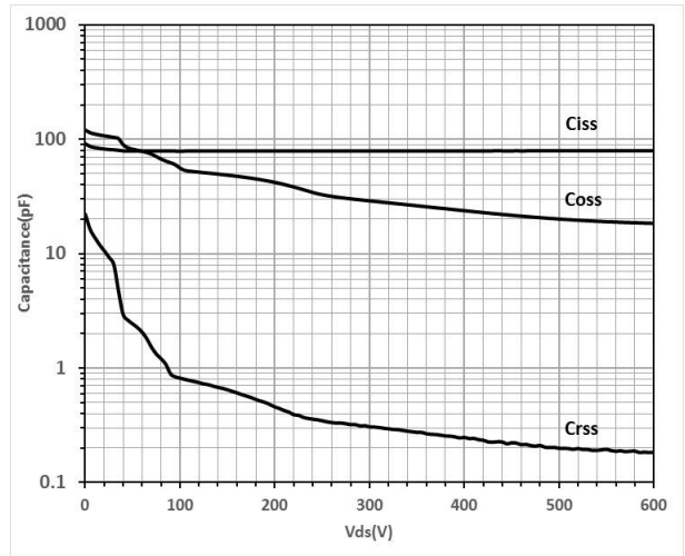
Figure 19 Typ. capacitances
