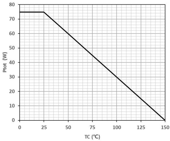
Figure 14 Power dissipation
