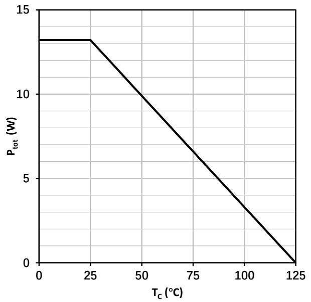
Figure 16 Power Dissipation
